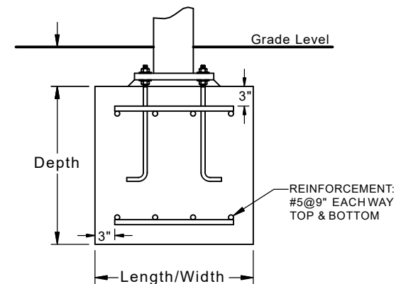
Typical Spread Footing
