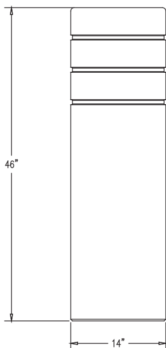
ELEVATION VIEW
