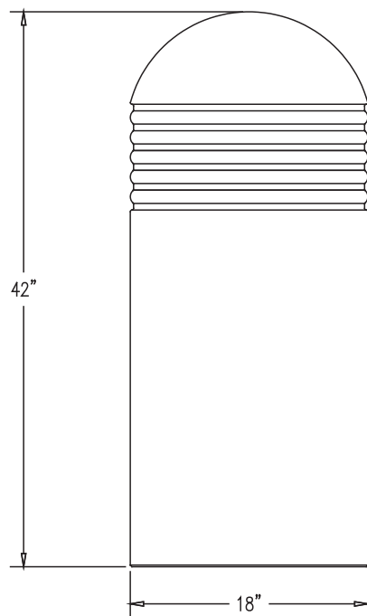
ELEVATION VIEW
