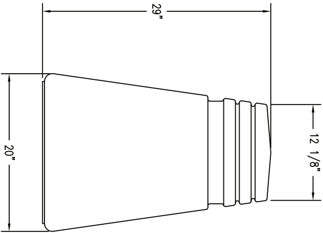
1 TOP VIEW
