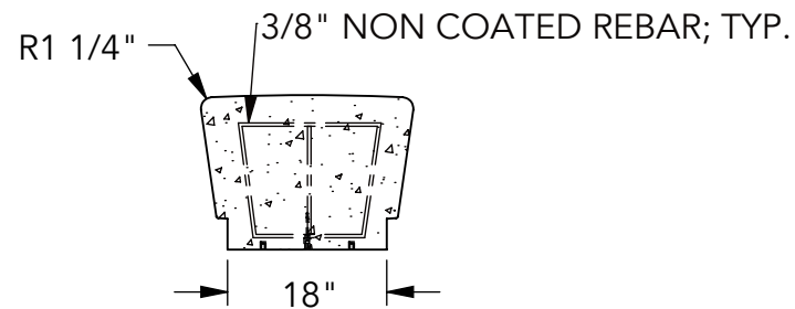
5 SECTION
