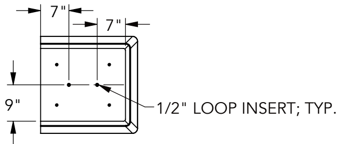
3 BOTTOM VIEW
