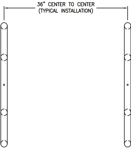
PLAN VIEW – TYPICAL INSTALLATION
