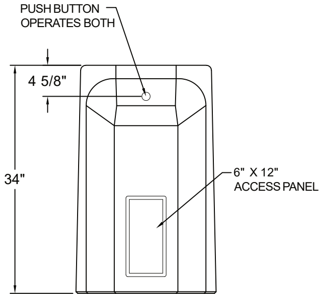
④ SIDE VIEW / FRONT VIEW
