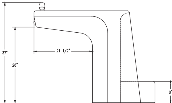
ELEVATION VIEW
