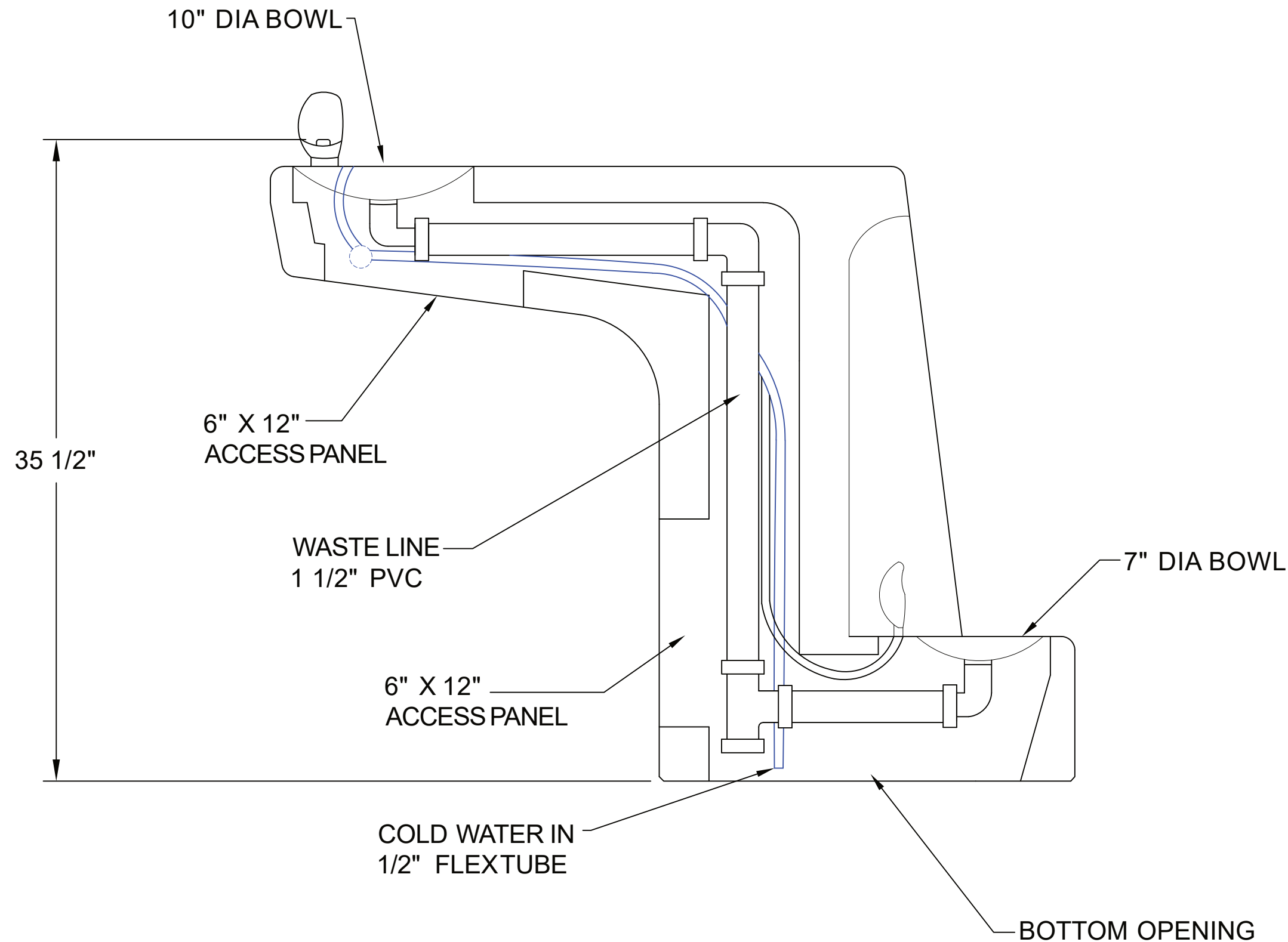
6 SECTION VIEW
